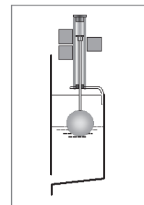
Electro-magnet gauges (FMR).
